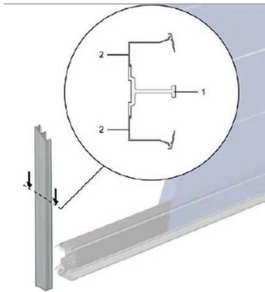
Guide rail 1. Guide rail 2. Seal angle
