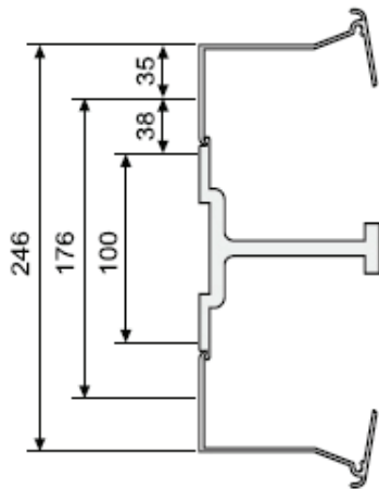
Screw hole distances in guide rails
