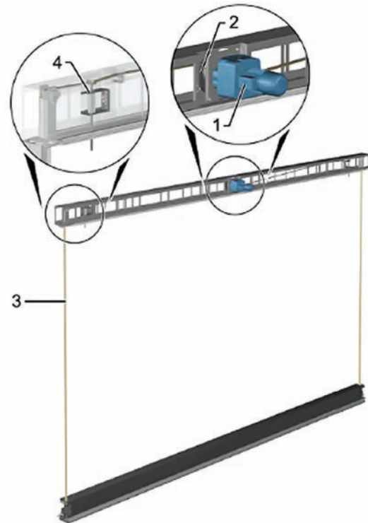
Header box 1. Drive unit 2. Belt drum 3. Lifting belt 4. Limit switching units
