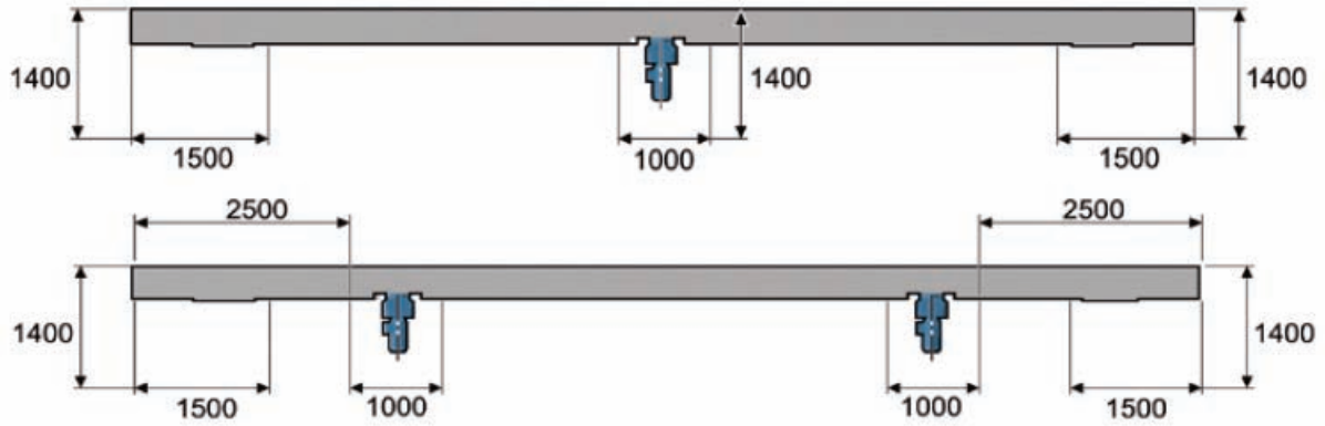
Space requirements for maintenance (mm)
